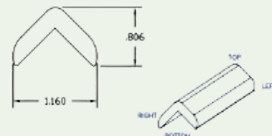
Corner Trim
