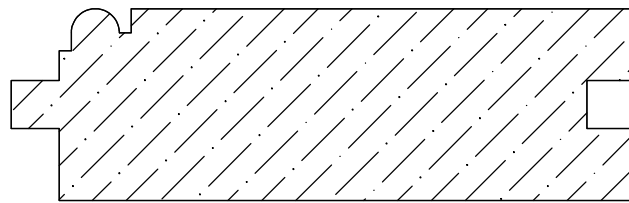
MP21-05 1 x 3 face *add 1/4 to get overall width
