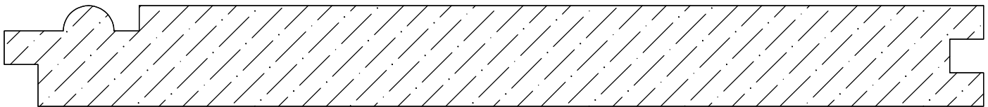
MP21-09 3/4 x 6-3/4 face *add 1/4 to get overall width
