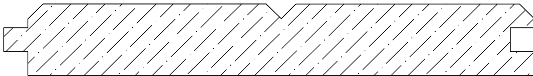
MP21-06 3/4 x 5-1/4 face *add 1/4 to get overall width
